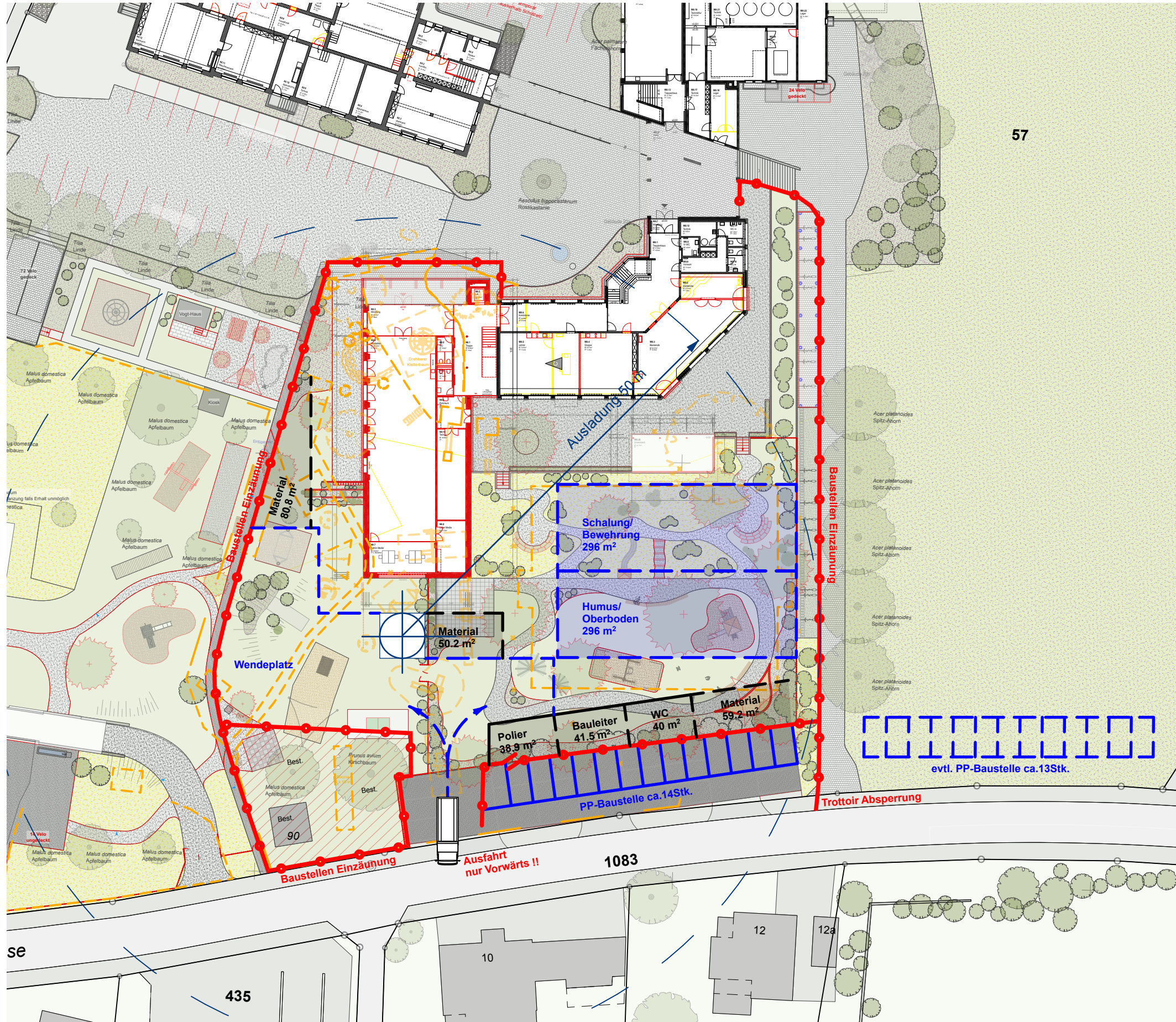
Situationsplan 1:500
